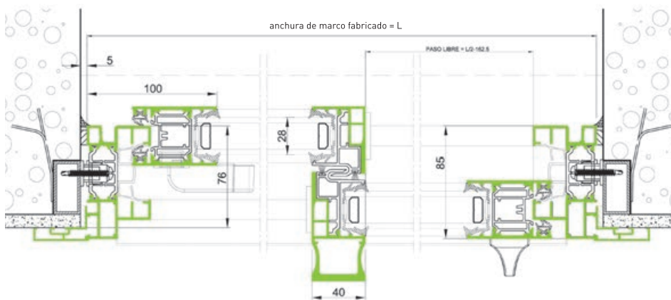
Corredera 2 railes
